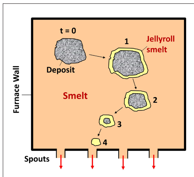
9. A postulated formation mechanism of jellyroll smelt by a fallen deposit.
