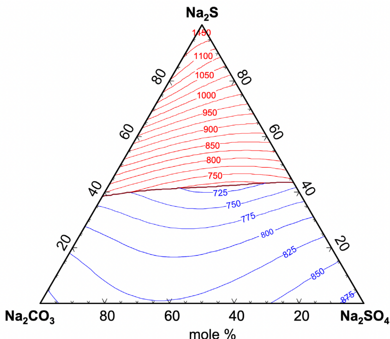
5. The sodium carbonate-sodium sulfide-sodium sulfate ( \text{Na}_2\text{CO}_3 - \text{Na}_2\text{S} - \text{Na}_2\text{SO}_4 ) phase diagram [7].
