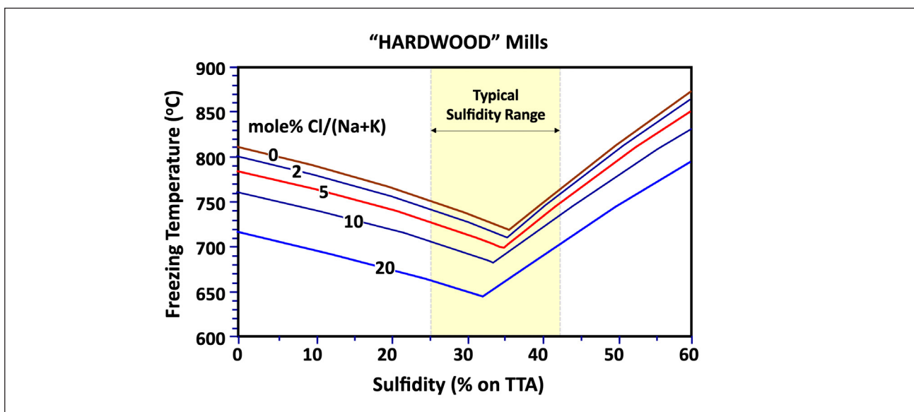
4. Effect of sulfidity on freezing temperature of molten smelt at different Cl contents for typical hardwood kraft mills with 10 mole% K/(Na+K) and 100% reduction efficiency.
