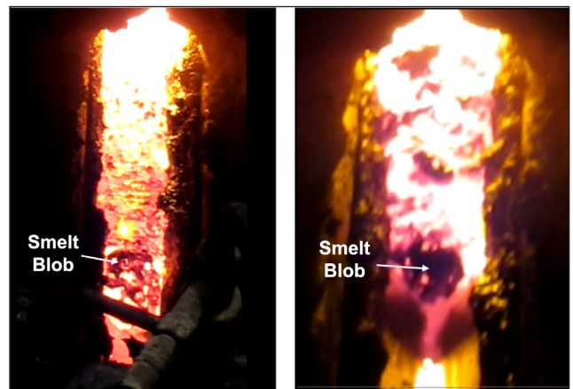
1. Jellyroll smelt blobs on spout troughs in two recovery boilers [1].
