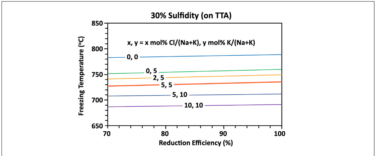
7. Effect of reduction efficiency on the freezing temperature of kraft smelt with 30% sulfidity and various Cl and K contents. Note that potassium contents of 5 mol% and 10 mol% K/(Na+K) are typical for softwood and hardwood liquors, respectively.
