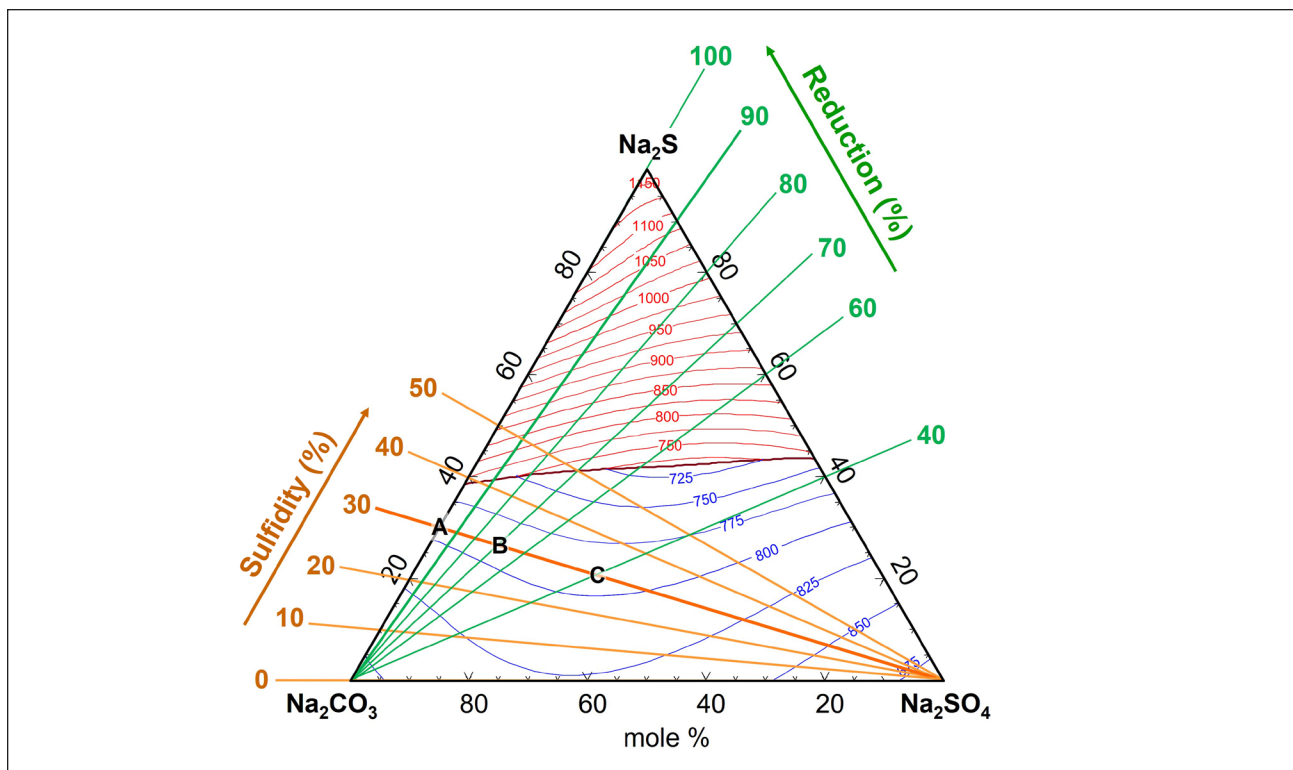
6. Iso-sulfidity and iso-reduction lines in the \text{Na}_2\text{CO}_3 - \text{Na}_2\text{S} - \text{Na}_2\text{SO}_4 phase diagram.
