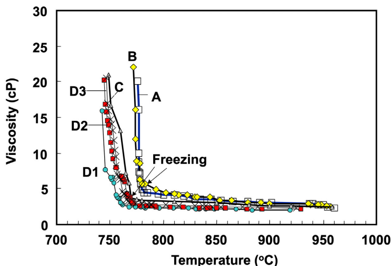
2. Viscosity of smelt samples from four kraft mills [6]. Each smelt sample has a slightly different composition and thus a different break point (first freezing temperature).
