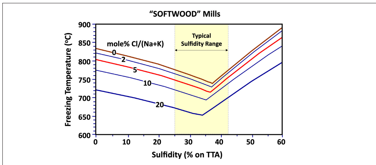
3. Effect of sulfidity on freezing temperature of molten smelt at different Cl contents for typical softwood kraft mills with 5 mole% K/(Na+K) and 100% reduction efficiency (Cl: chloride; K: potassium; Na: sodium).
