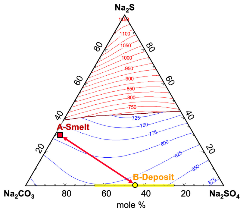
8. Change in freezing temperatures of smelt/fallen deposit mixtures in the \text{Na}_2\text{CO}_3\text{-Na}_2\text{S-Na}_2\text{SO}_4 phase diagram.
